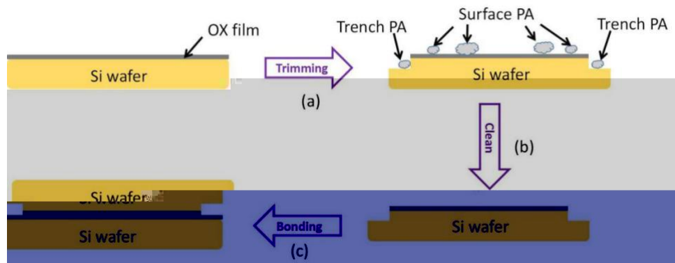
Fig. 1: Schematic illustration of Xtacking 3D NAND bonding trimming process: (a) Trimming; (b) Clean; (c) Bonding
