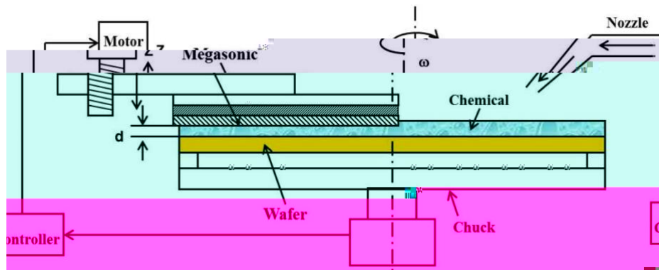
Fig 3: Wafer cleaning apparatus using SAPS megasonic device
